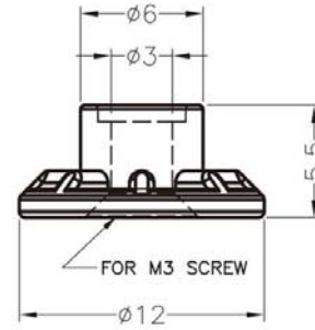
MOUNTING HOLE ø6
