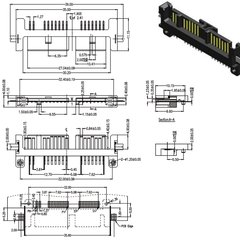
Recommended PCB Layout (PCB TOLERANCE \pm 0.05 )
