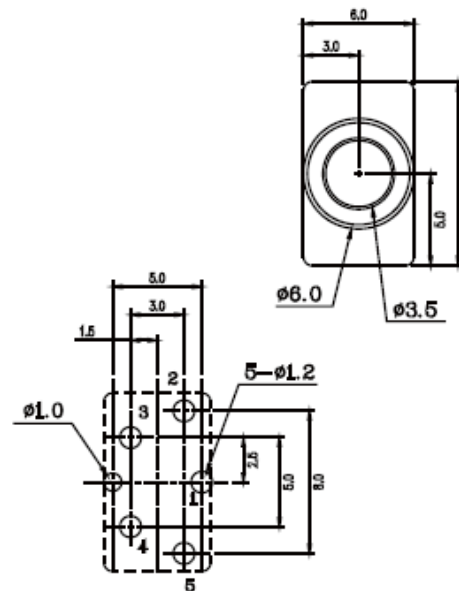
Recommended PCB Layout (PCB TOLERANCE \pm 0.05 )
