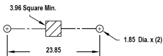
PCB Layout
