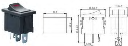
A-TOP1-3-101EN ON-OFF (3V LED)
