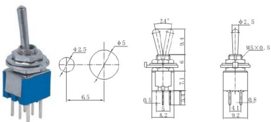
BTS-202-A2 ON-ON DPDT 6P
