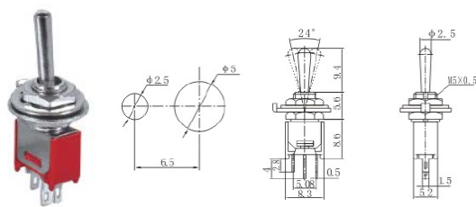
BTS-103-2A1 ON-OFF-ON SPDT 3P
