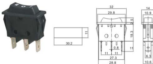
A-TOP3-4-103 ON-OFF-ON A-TOP3-4-123 (ON)-OFF-(ON)
