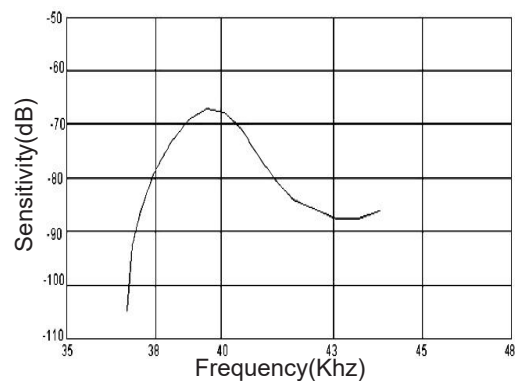
SPL-Frequency Characteristics
