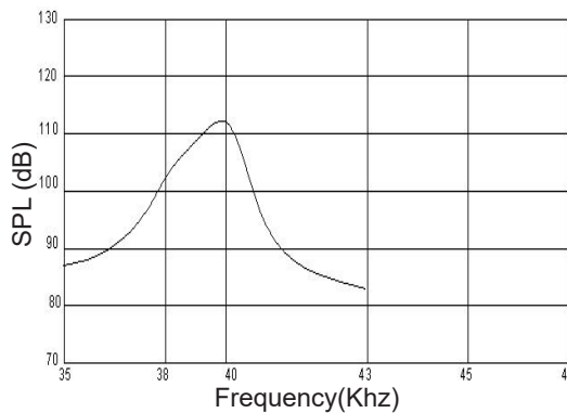
SPL-Frequency Characteristics
