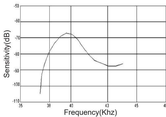
SPL-Frequency Characteristics
