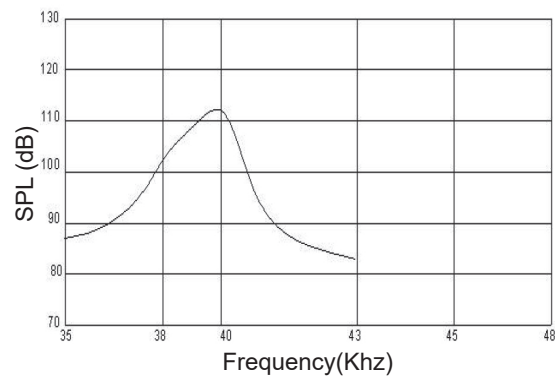
SPL-Frequency Characteristics
