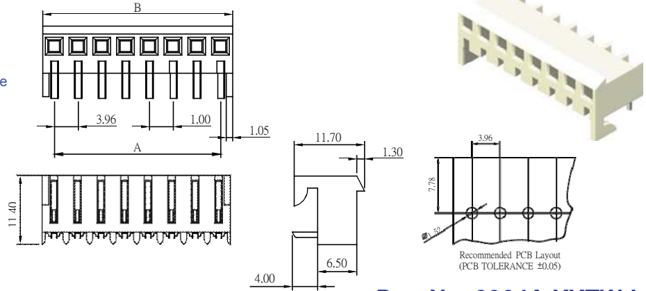
Part No.:3964A-XXTW-L
