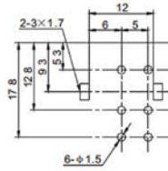
P.C.B LAYOUT (VIEWED FROM COPPER SIDE)
