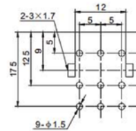
P.C.B LAYOUT (VIEWED FROM COPPER SIDE)
