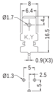
MOUNTINGHOLES
