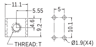
MOUNTING HOLES
