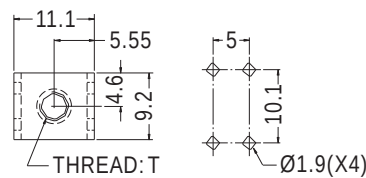
MOUNTING HOLES
