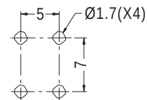
MOUNTING HOLES
