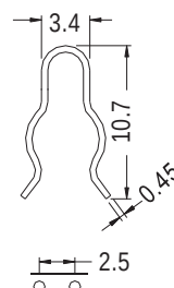
MOUNTING HOLES HOLE IN P.C.B Ø0.8~Ø1.0
