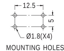
MOUNTING HOLES
