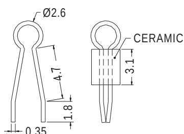
TEST-3S HOLE IN P.C.B Ø0.8~Ø1.0
