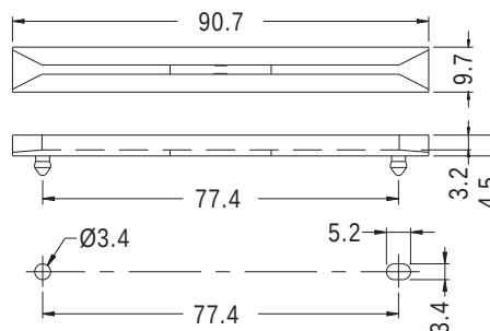
MOUNTING HOLES
