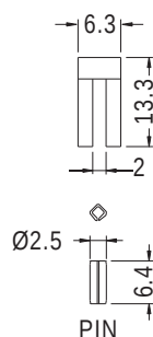
MOUNTING HOLE
