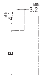
TYPICAL BOARD CUT-OUT
