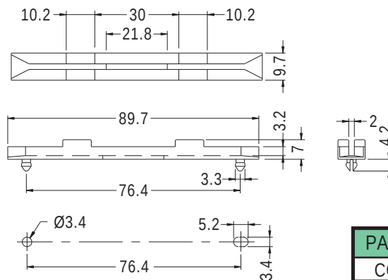
MOUNTING HOLES
