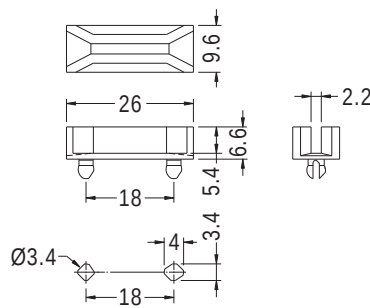
MOUNTING HOLES
