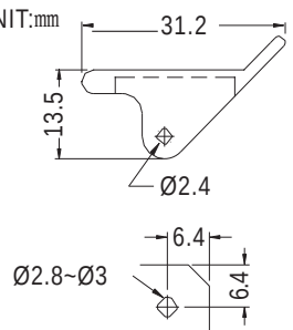
MOUNTING HOLE
