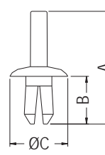
CHASSIS: ØD THICKNESS: E FOR PSR5.5-10S
