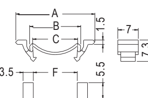
MOUNTING HOLES FOR CCMB-15, CCMB-30
