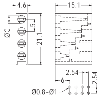
MOUNTING HOLES
