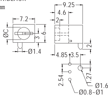
MOUNTING HOLES
