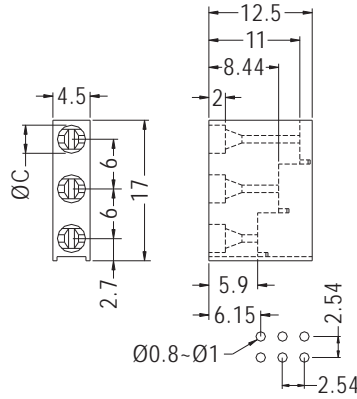
MOUNTING HOLES
