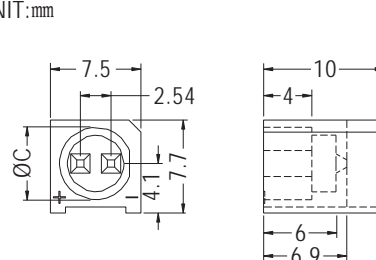
MOUNTING HOLES
