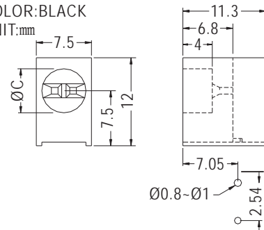
MOUNTING HOLES
