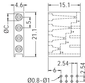
MOUNTING HOLES
