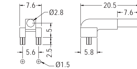
MOUNTING HOLES
