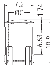
CHASSIS Ø6.4-Ø6.45 THICKNESS 0.8-6.35
