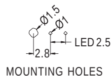
MOUNTING HOLES
