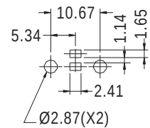
MOUNTING HOLES
