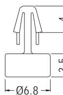
P.C.B Ø3.0 THICKNESS 3.0
